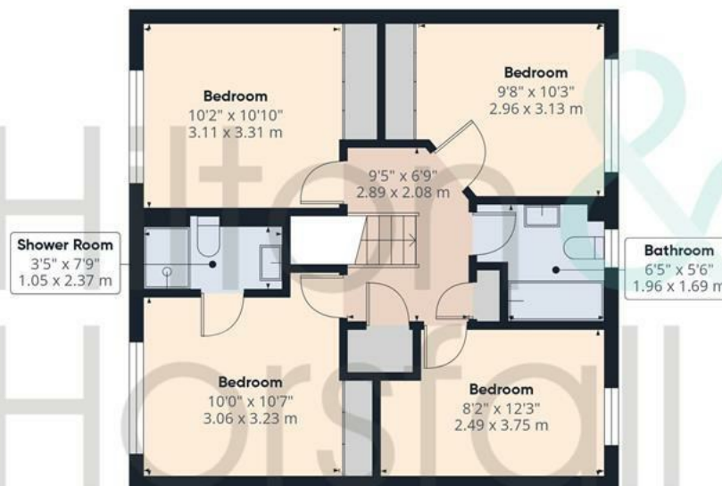
Floor 1
